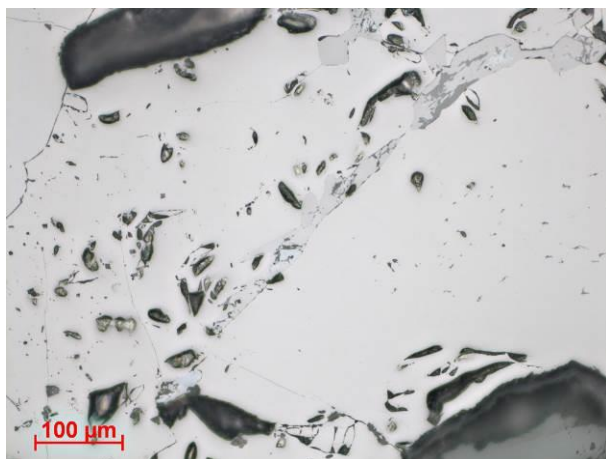
Figure 6.9 Left: Massive magnetite (white), hematite (lighter) and ilmenite (darker) occur as fissure filling (RL PPL). Right: Massive magnetite grain (white) with ilmenite (grey) developed at a fissure (RL PPL).
