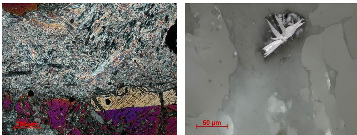
Figure 6.4 Left: Twinned diopside crystals (bottom) fragmented and accompanied by acicular talc (TL XPL). Right: Tiny molybdenite crystals in calcite (RL PPL).
